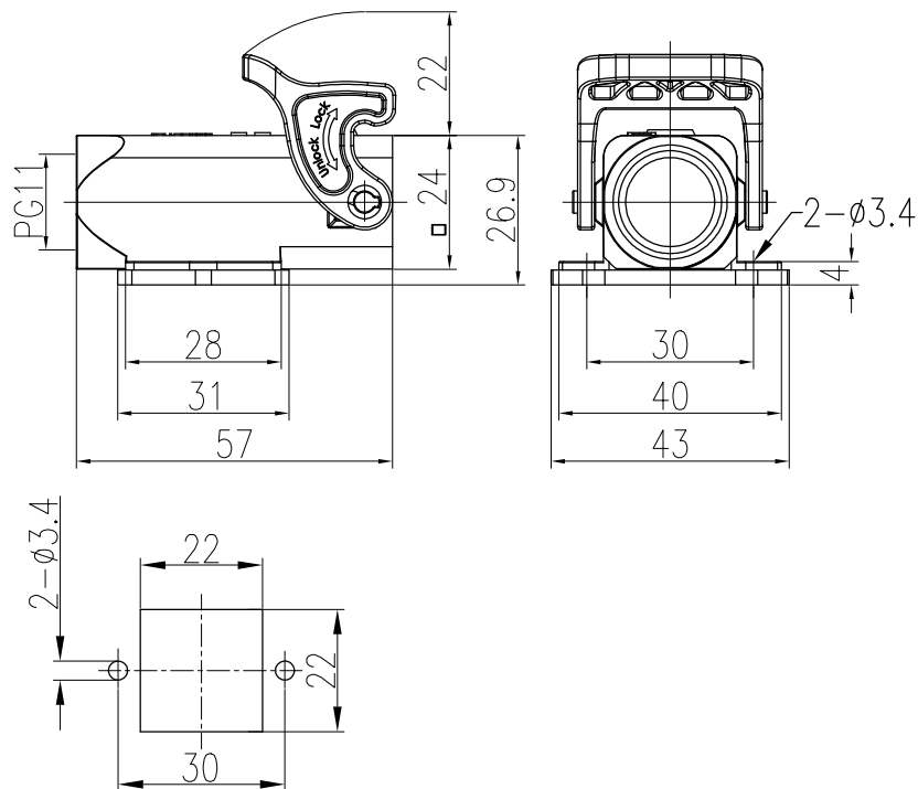
面板开孔图 Panel cut out
